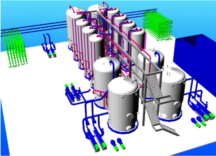
Digelys Turbo™ - Boosted Anaerobic Digestion (THP Process)
