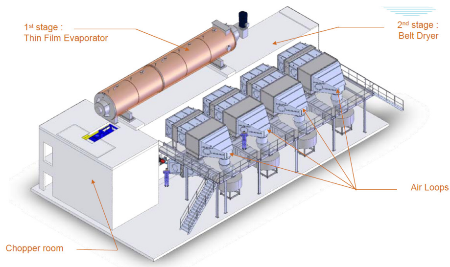
Evaporis LE™ - Low Energy Thermal Dryer
