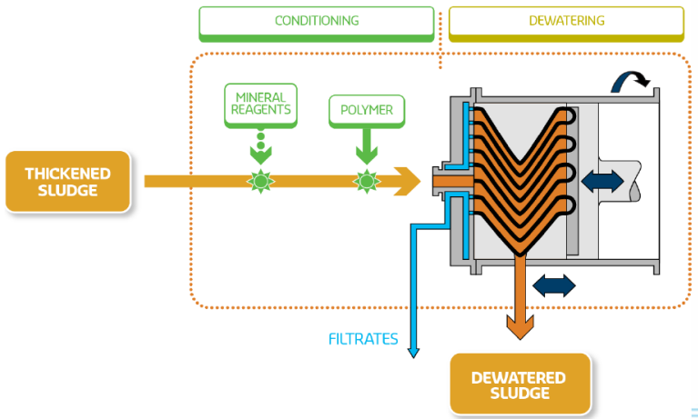
Dehydris Twist™ (Bucher Piston Press) for Sludge Dewatering
